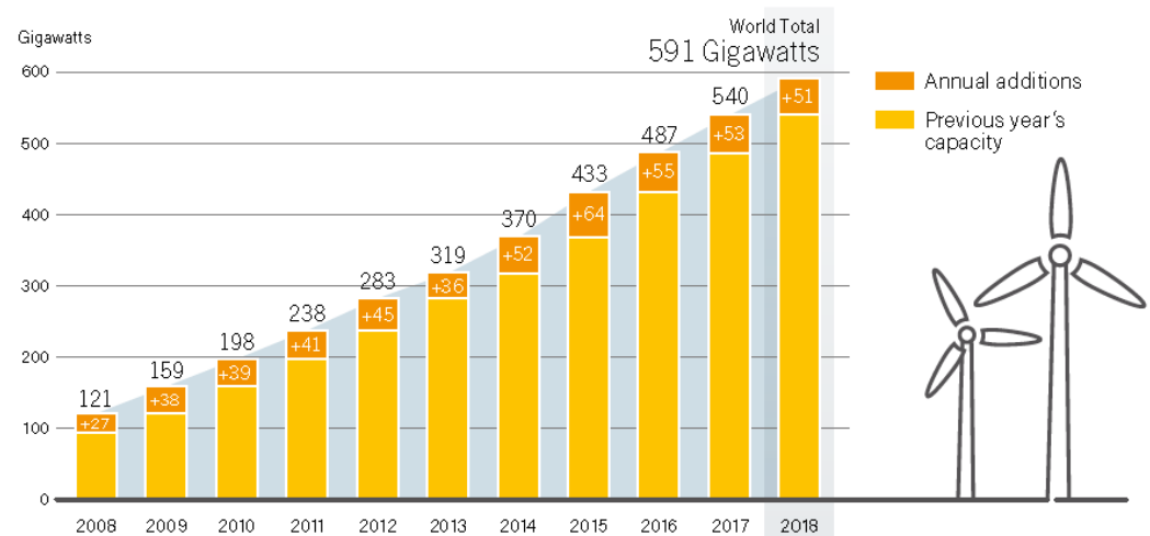
FIGURE 35. Wind Power Global Capacity and Annual Additions, 2008-2018
